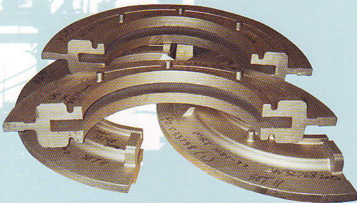
SEAL JOINTS FOR PROPELLER SHAFTS
